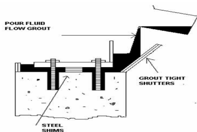
Figure 1. Grout shutter detail
