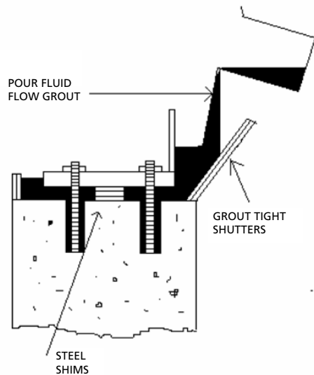
Figure 1. Grout shutter detail
