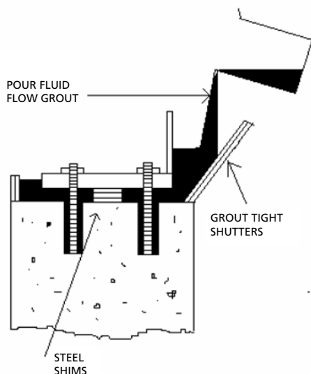
Figure 1. Grout shutter detail
